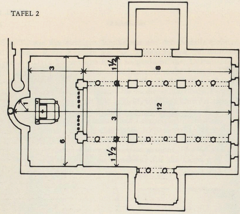
Plan B: S. Maria in Portico, modular plan (not drawn to scale).
