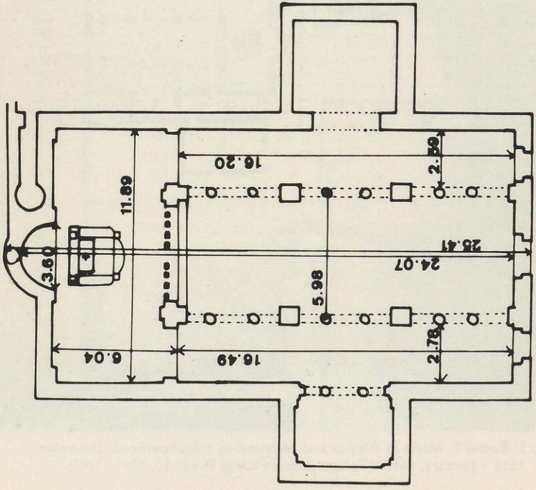
Plan A: S. Maria in Portico, plan (not drawn to scale) with dimensions marked.
